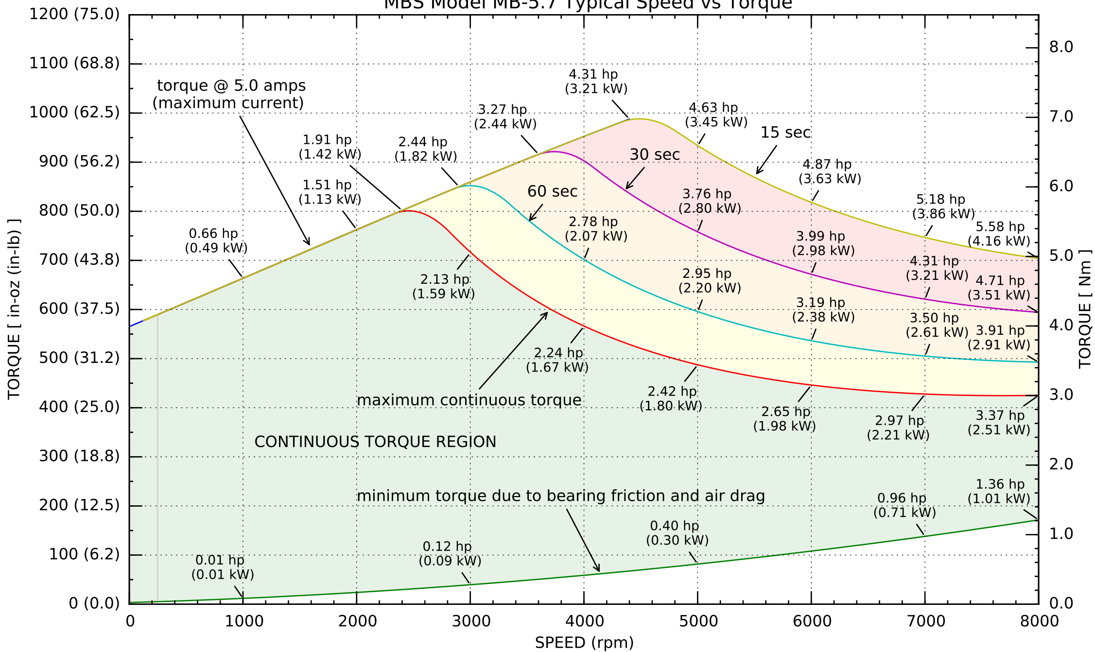
MBS Model MB-5.7 Typical Speed vs Torque
