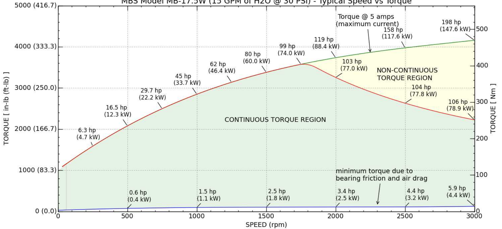
MBS Model MB-17.5W (15 GPM of H2O @ 30 PSI) - Typical Speed vs Torque
