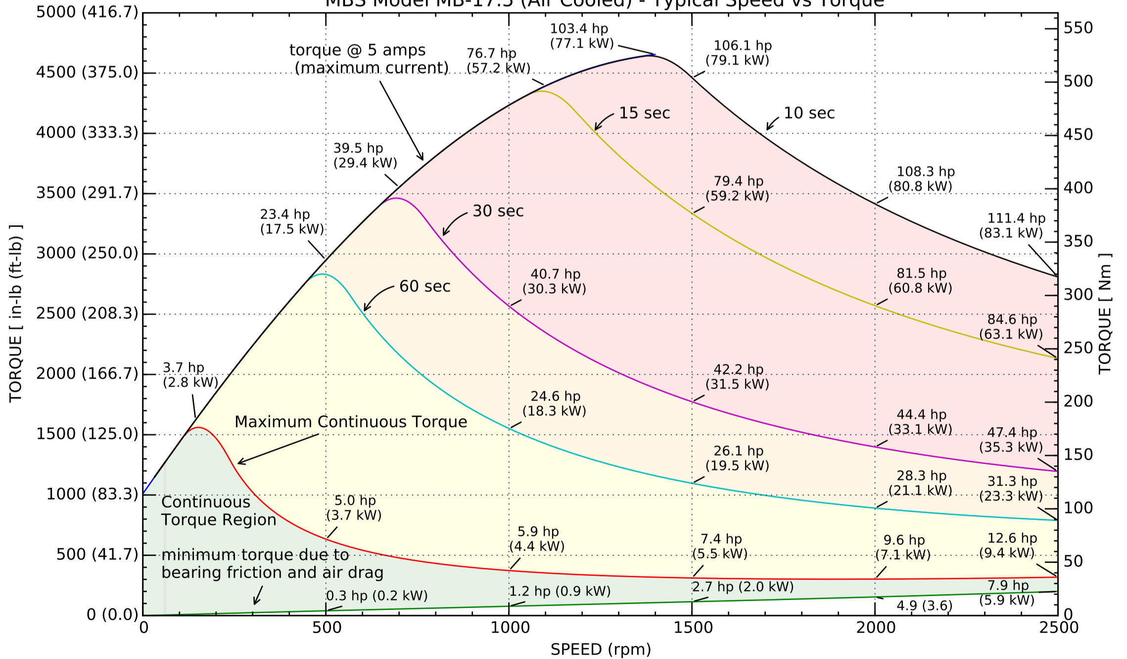
MBS Model MB-17.5 (Air Cooled) - Typical Speed vs Torque
